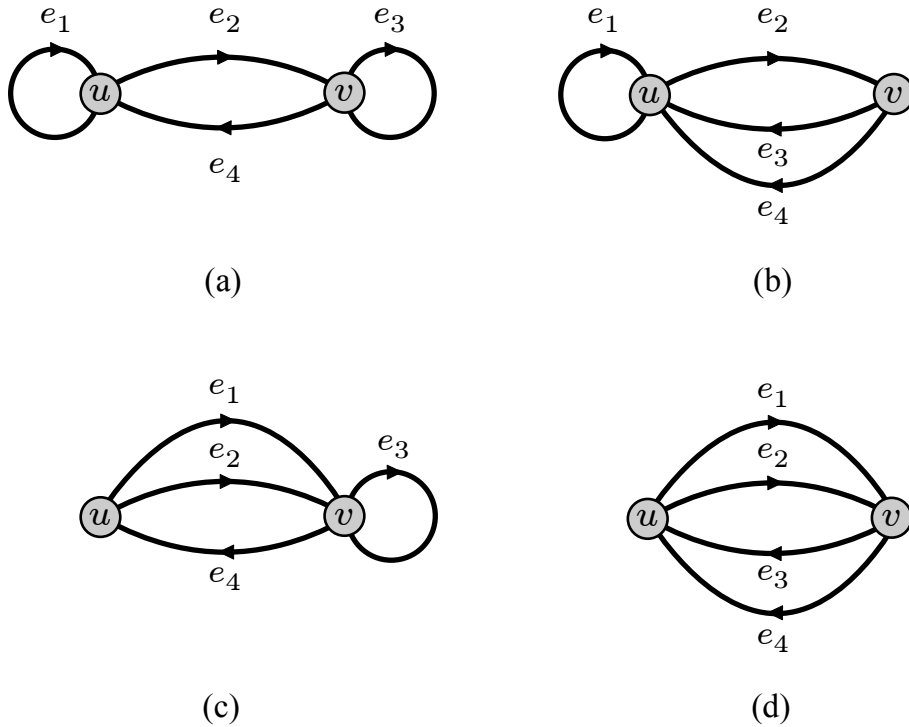
Figure. 2.6.3: The four minimal graphs for 2-vertex directed graph IFSs.
