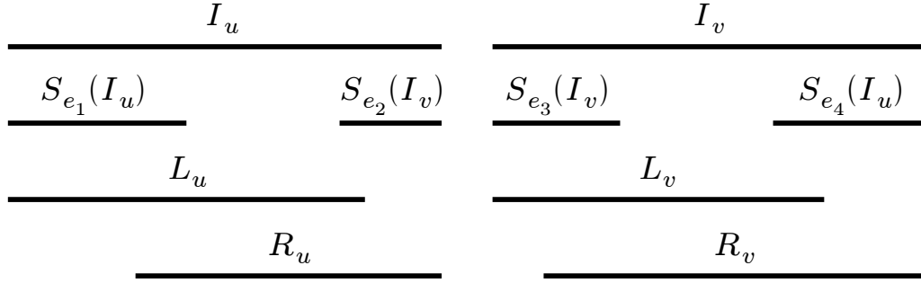
Figure 3.4.3: Some possibilities for the intervals L_u , L_v , R_u , and R_v .
