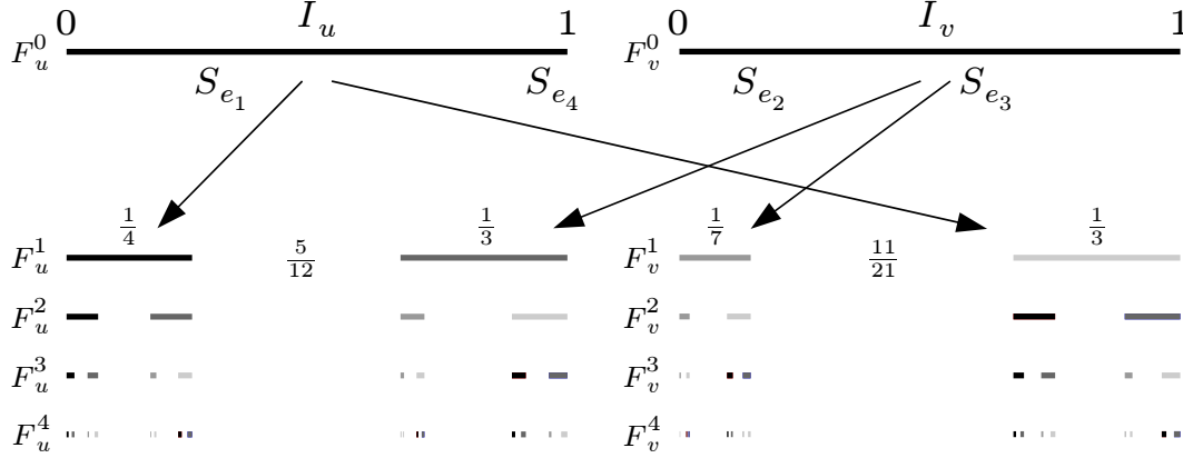
Figure 7.1: Level- k intervals for 0 \leq k \leq 4 .
