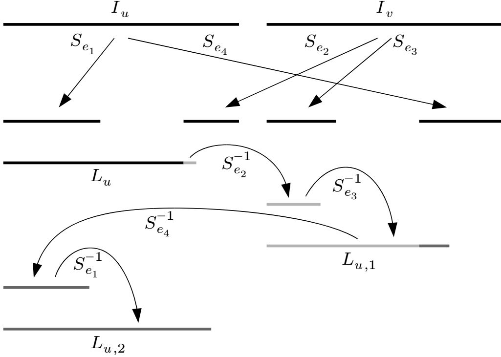
Figure 4.4: The intervals L_u , L_{u,1} , and L_{u,2} .
