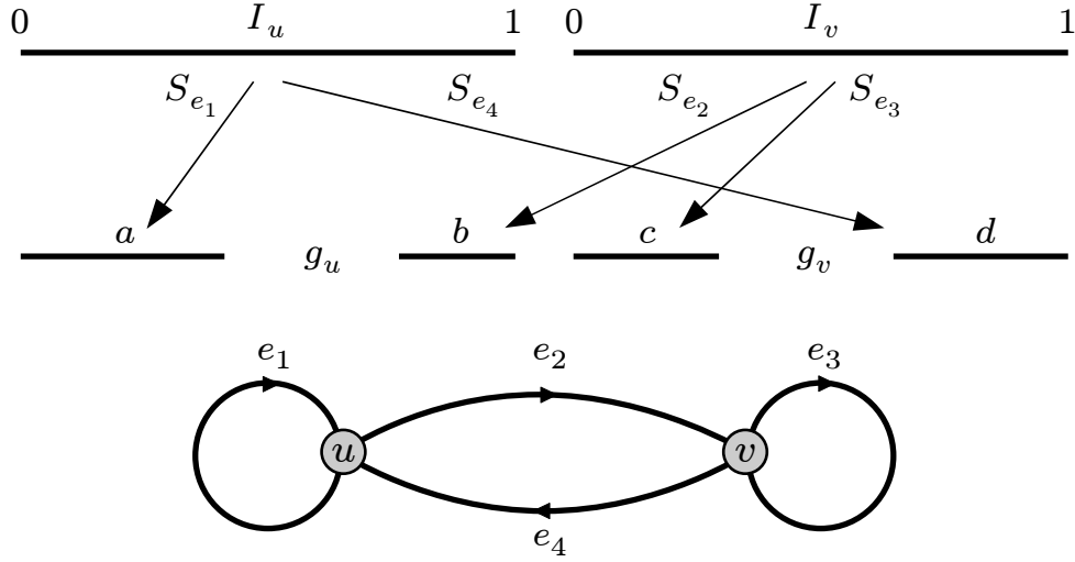
Figure 4.5: A 2-vertex directed graph IFS defined on the unit interval, the similarities S_{e_1} , S_{e_2} , S_{e_3} and S_{e_4} do not reflect.
