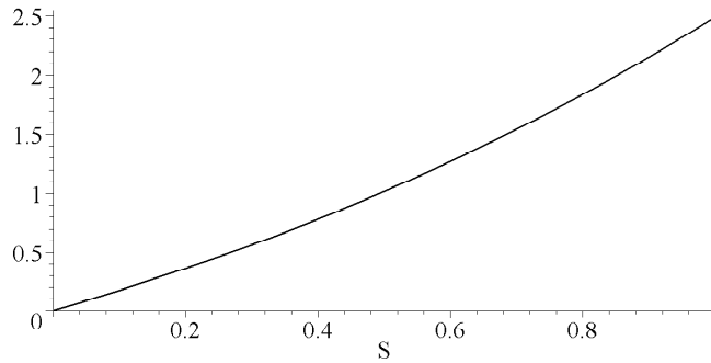
Figure 4.6: A plot of \frac{(a+g_u)(|I_u|^s - a^s)}{b a^s} .
