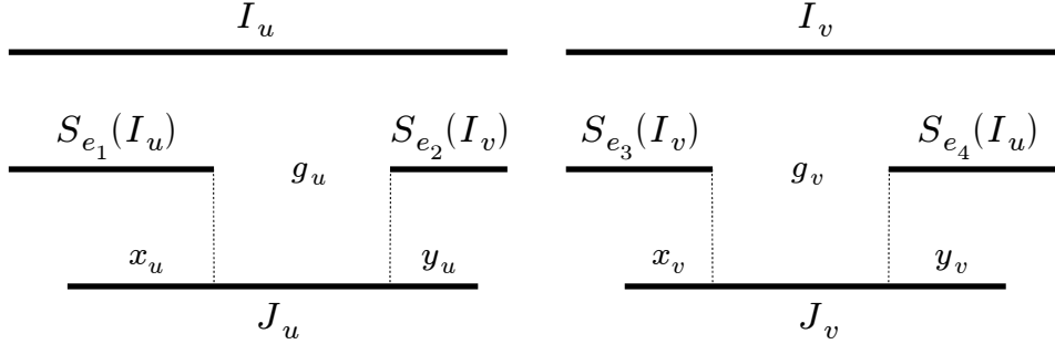
Figure 4.2: The intervals J_u and J_v .
